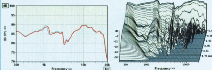
ABOVE LEFT: A 'switchback' frequency response with a significant notch in output between 3-5kHz; ABOVE RIGHT: Resonances at 1kHz and 3kHz are probably associated with breakup modes in the midrange driver
